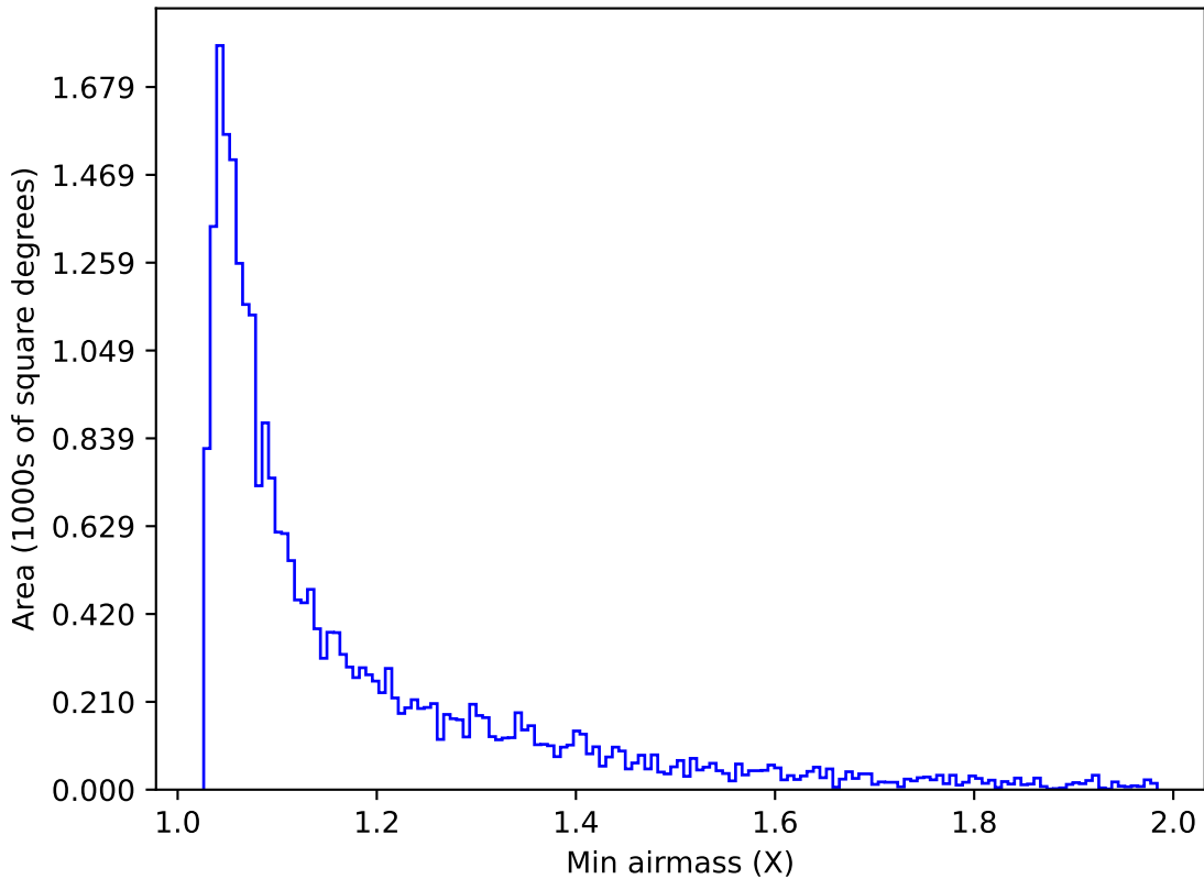
too_elab_r32_d2_gz_v3.4_10yrs Yr 1 g band: Min airmass
