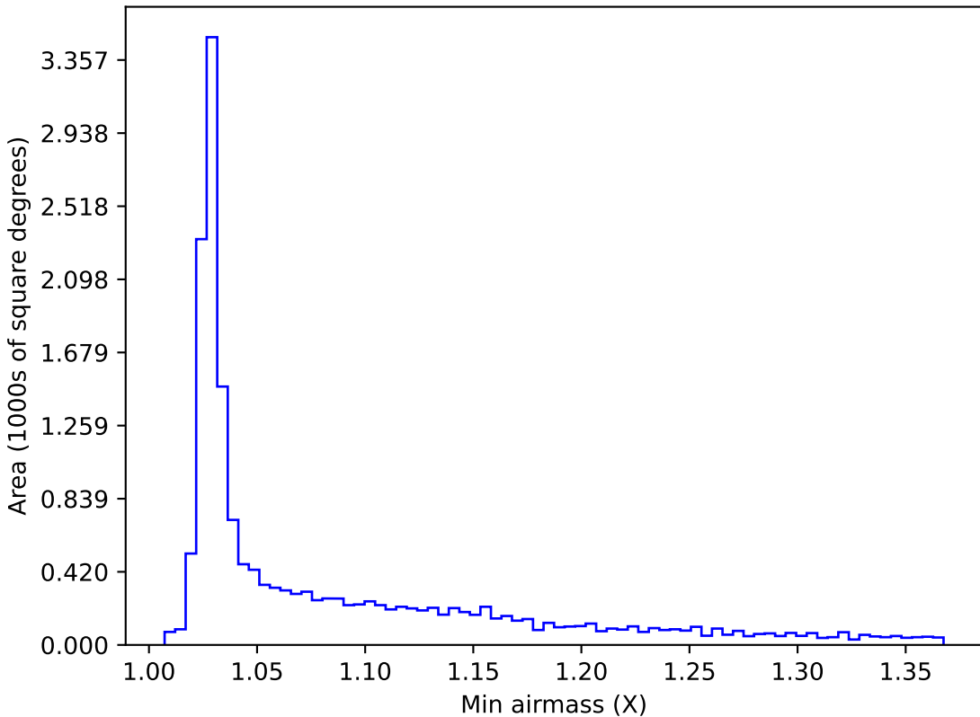
too_elab_r32_d2_gz_v3.4_10yrs WFD z band: Min airmass
