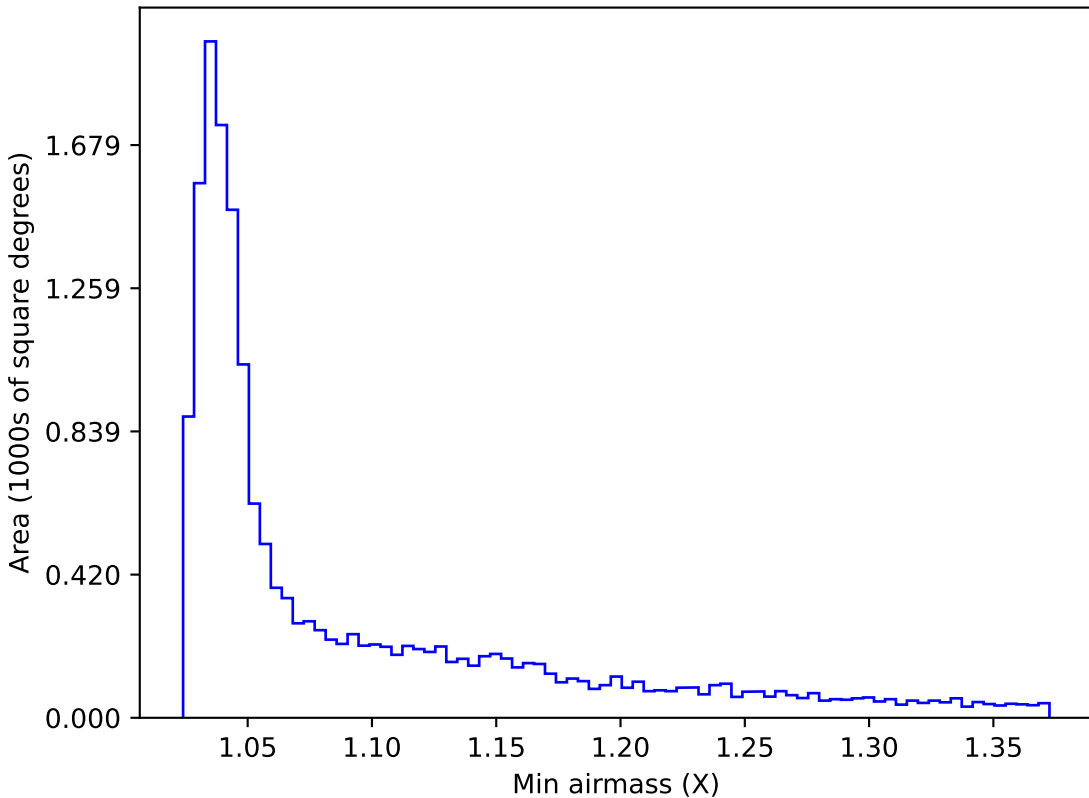
too_elab_r32_d2_gz_v3.4_10yrs WFD u band: Min airmass
