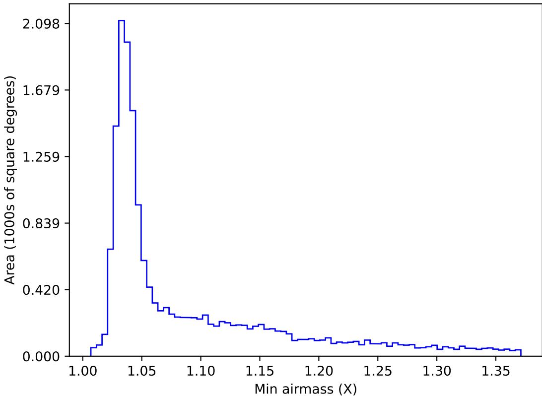
too_elab_r32_d2_gz_v3.4_10yrs WFD g band: Min airmass
