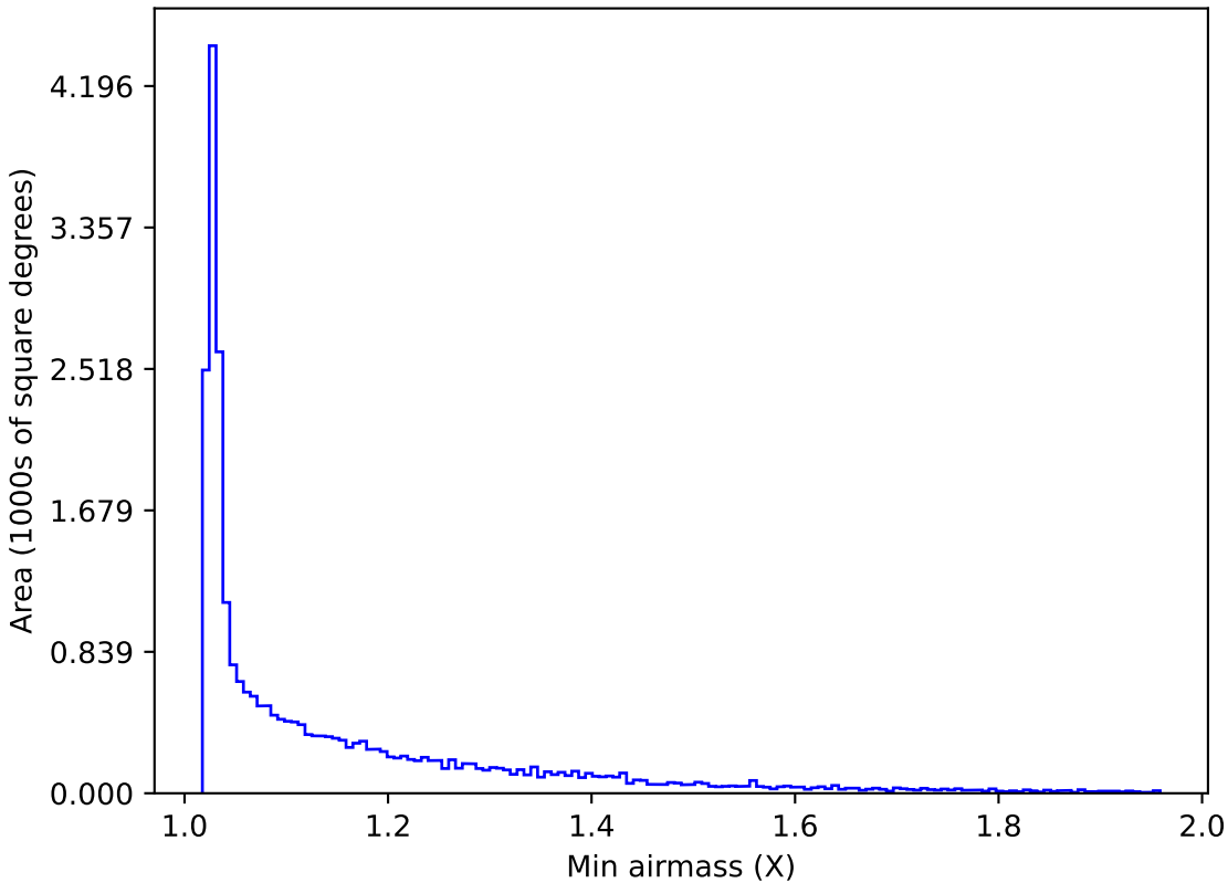
too_elab_r32_d2_gz_v3.4_10yrs All sky r band: Min airmass
