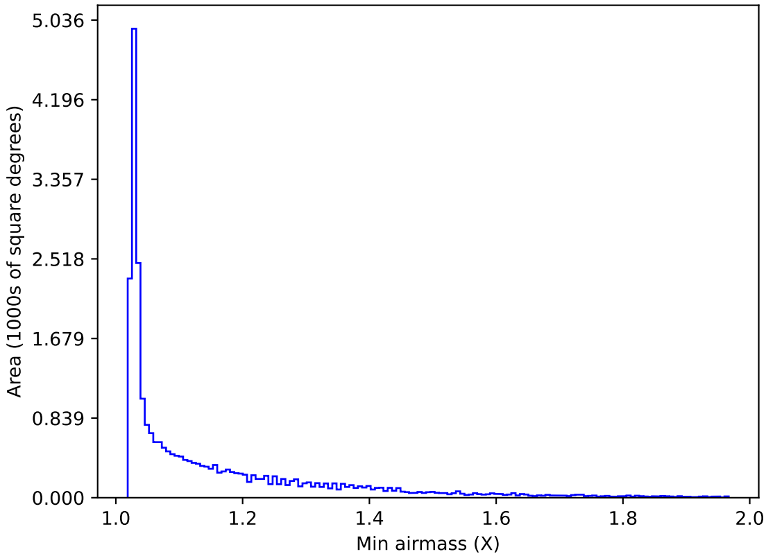
too_elab_r32_d2_gz_v3.4_10yrs All sky i band: Min airmass
