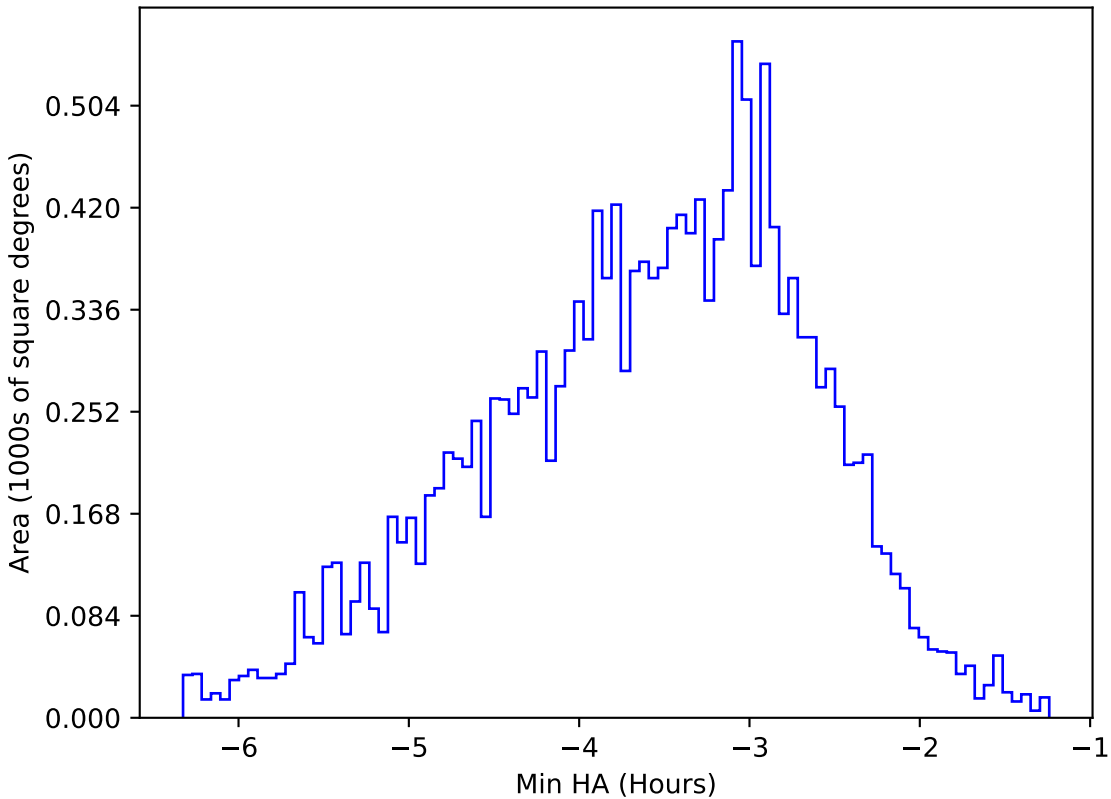
too_elab_r32_d2_gz_v3.4_10yrs WFD y band: Min HA
