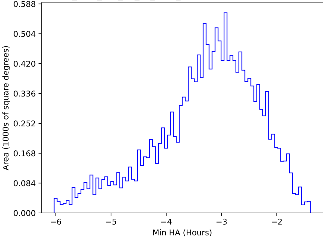
too_elab_r32_d2_gz_v3.4_10yrs WFD u band: Min HA
