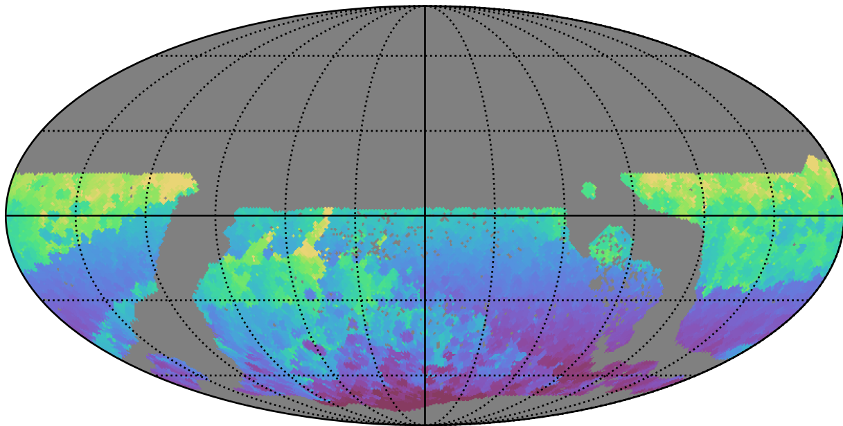
too_elab_r32_d2_gz_v3.4_10yrs WFD r band: Min HA
