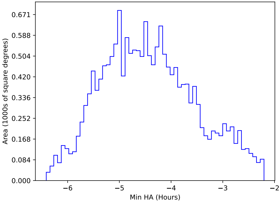
too_elab_r32_d2_gz_v3.4_10yrs WFD r band: Min HA
