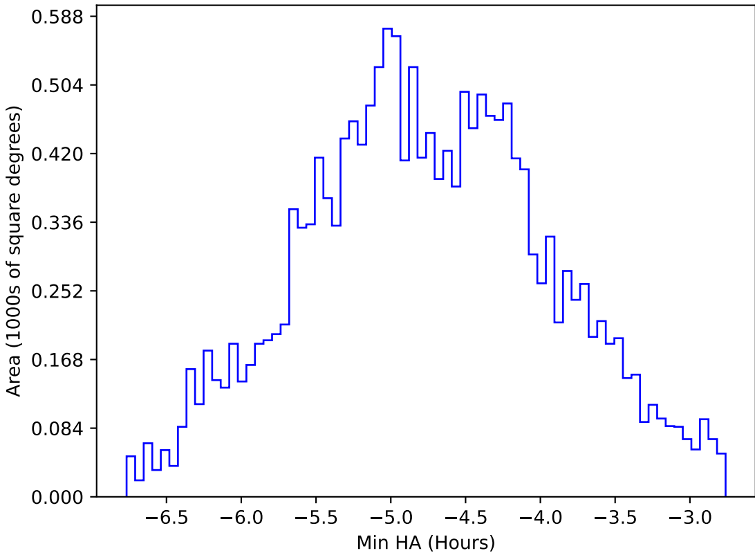
too_elab_r32_d2_gz_v3.4_10yrs WFD all bands: Min HA
