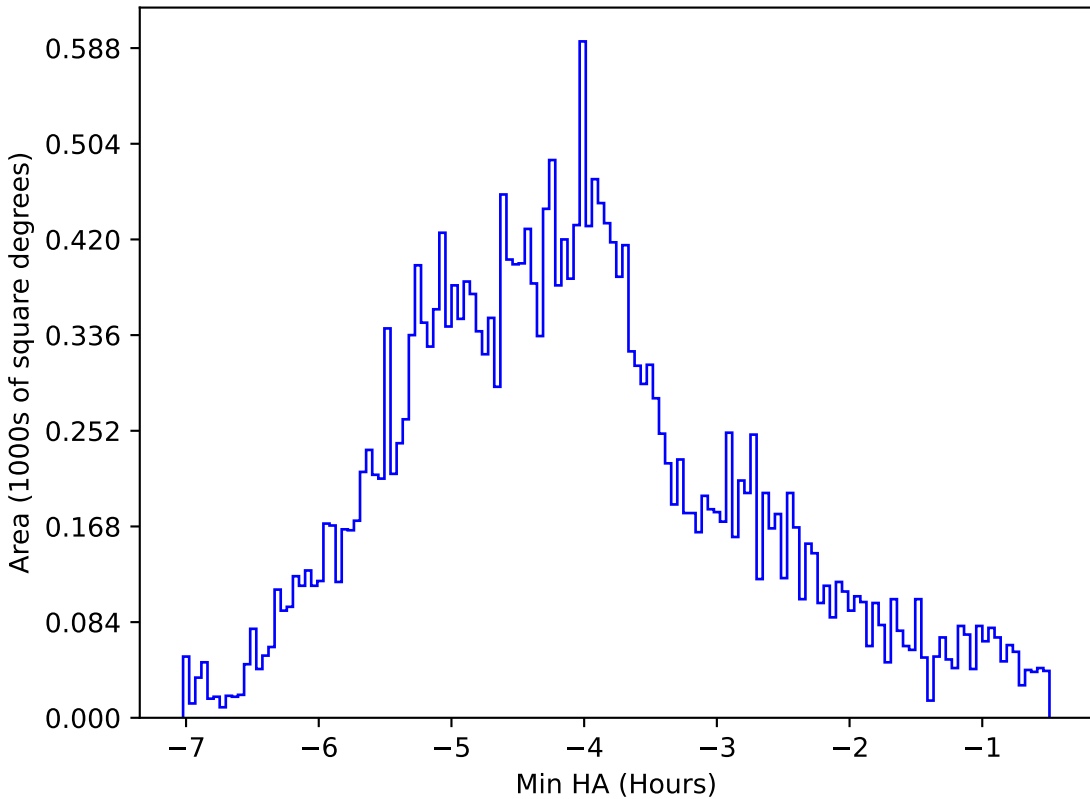
too_elab_r32_d2_gz_v3.4_10yrs All sky z band: Min HA
