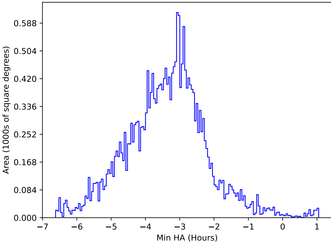
too_elab_r32_d2_gz_v3.4_10yrs All sky y band: Min HA
