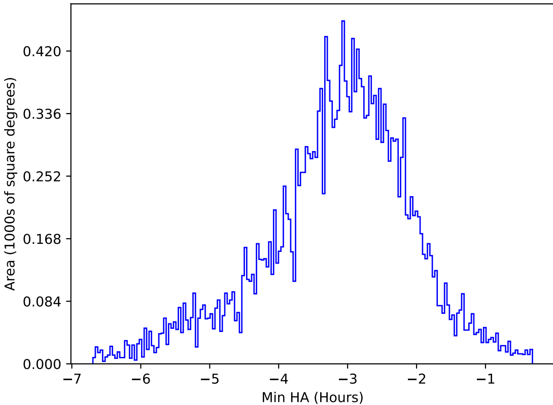
too_elab_r32_d2_gz_v3.4_10yrs All sky u band: Min HA
