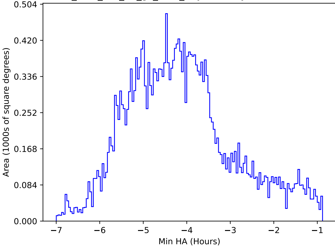
too_elab_r32_d2_gz_v3.4_10yrs All sky r band: Min HA
