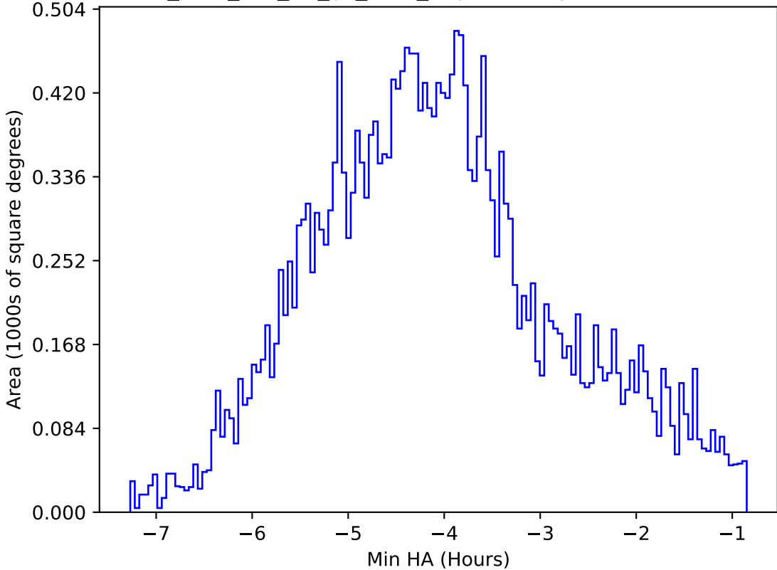
too_elab_r32_d2_gz_v3.4_10yrs All sky i band: Min HA
