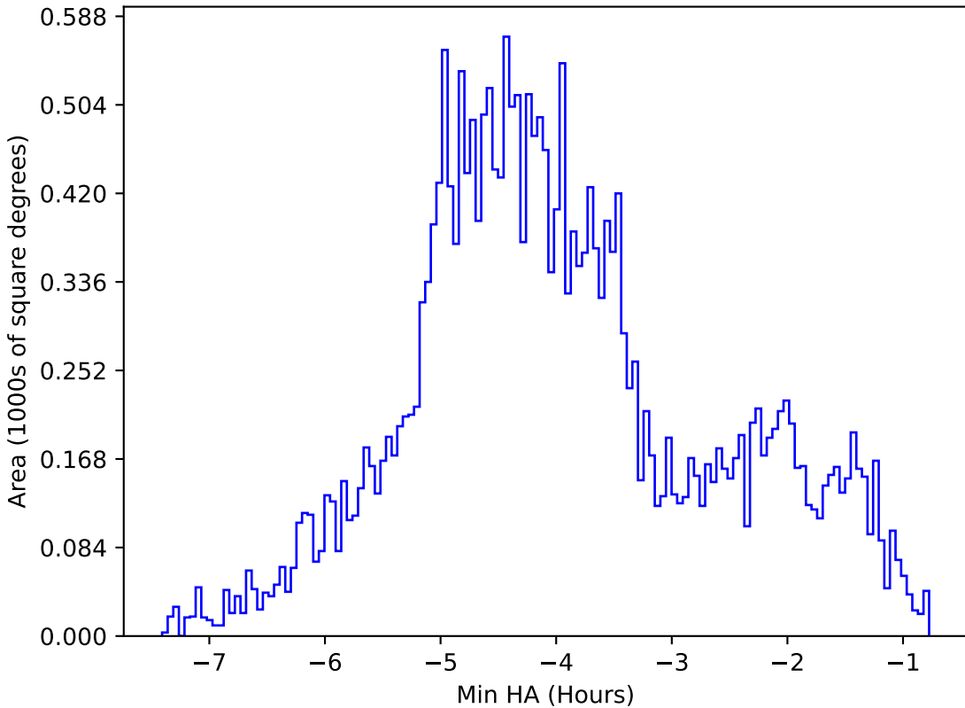
too_elab_r32_d2_gz_v3.4_10yrs All sky g band: Min HA
