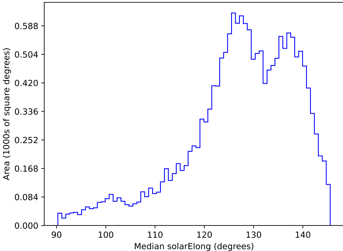
too_elab_r32_d2_gz_v3.4_10yrs WFD z band: Median solarElong
