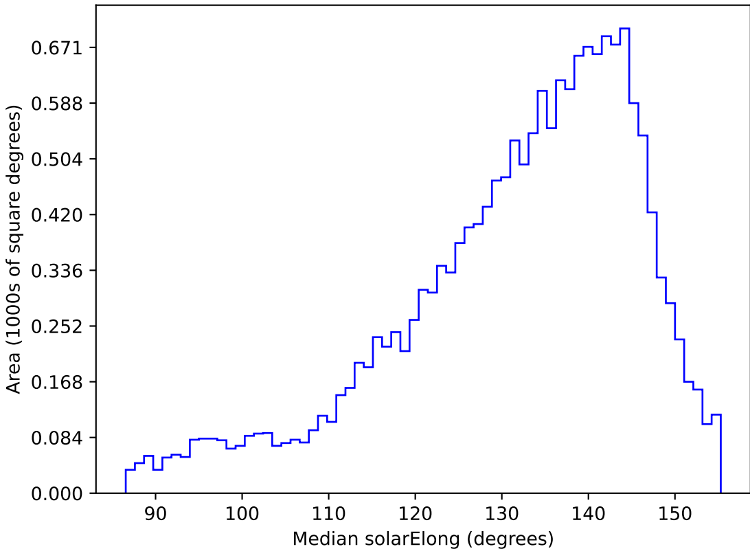
too_elab_r32_d2_gz_v3.4_10yrs WFD u band: Median solarElong
