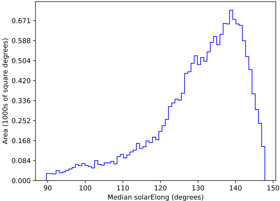
too_elab_r32_d2_gz_v3.4_10yrs WFD r band: Median solarElong
