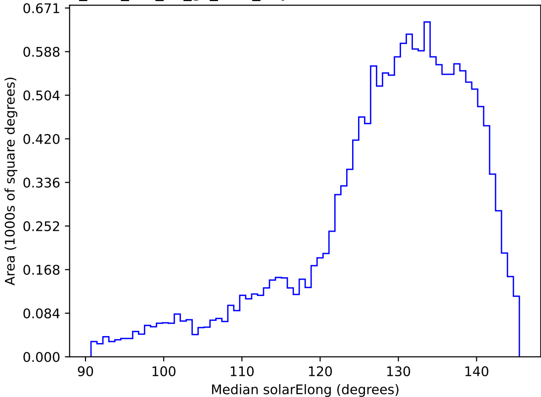
too_elab_r32_d2_gz_v3.4_10yrs WFD i band: Median solarElong
