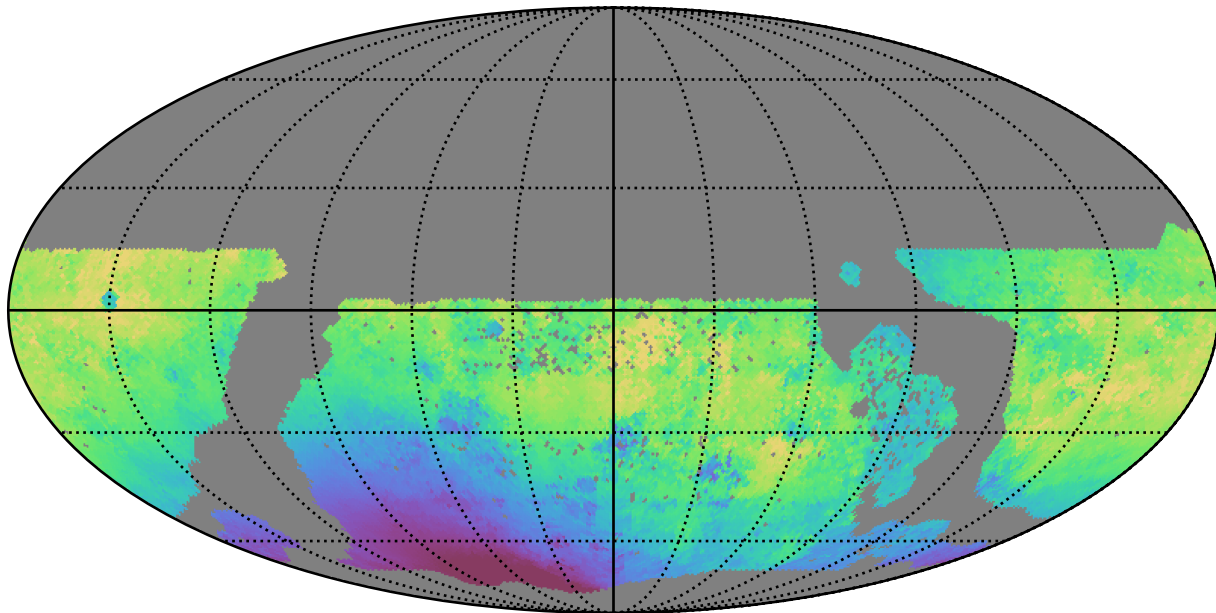
too_elab_r32_d2_gz_v3.4_10yrs WFD g band: Median solarElong
