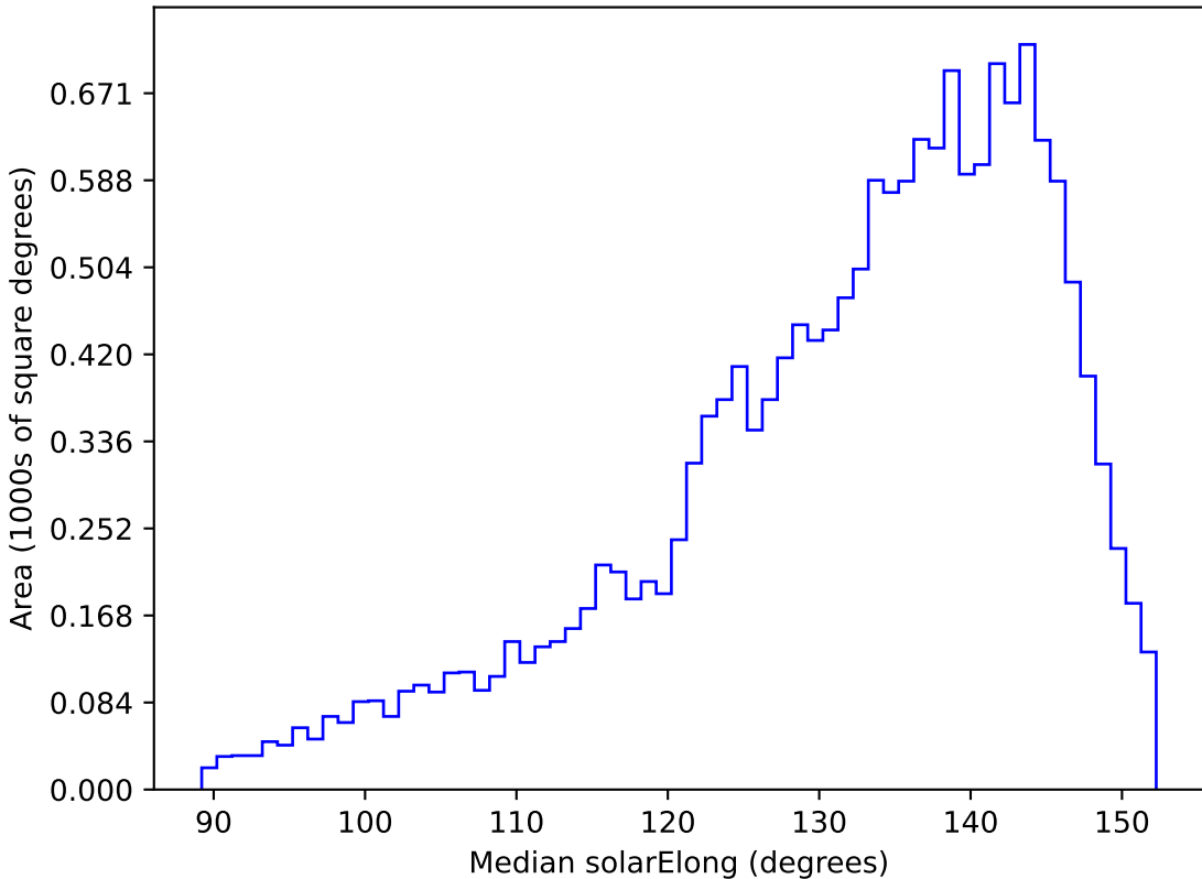
too_elab_r32_d2_gz_v3.4_10yrs WFD g band: Median solarElong
