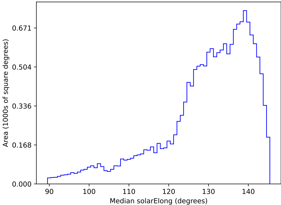
too_elab_r32_d2_gz_v3.4_10yrs WFD all bands: Median solarElong
