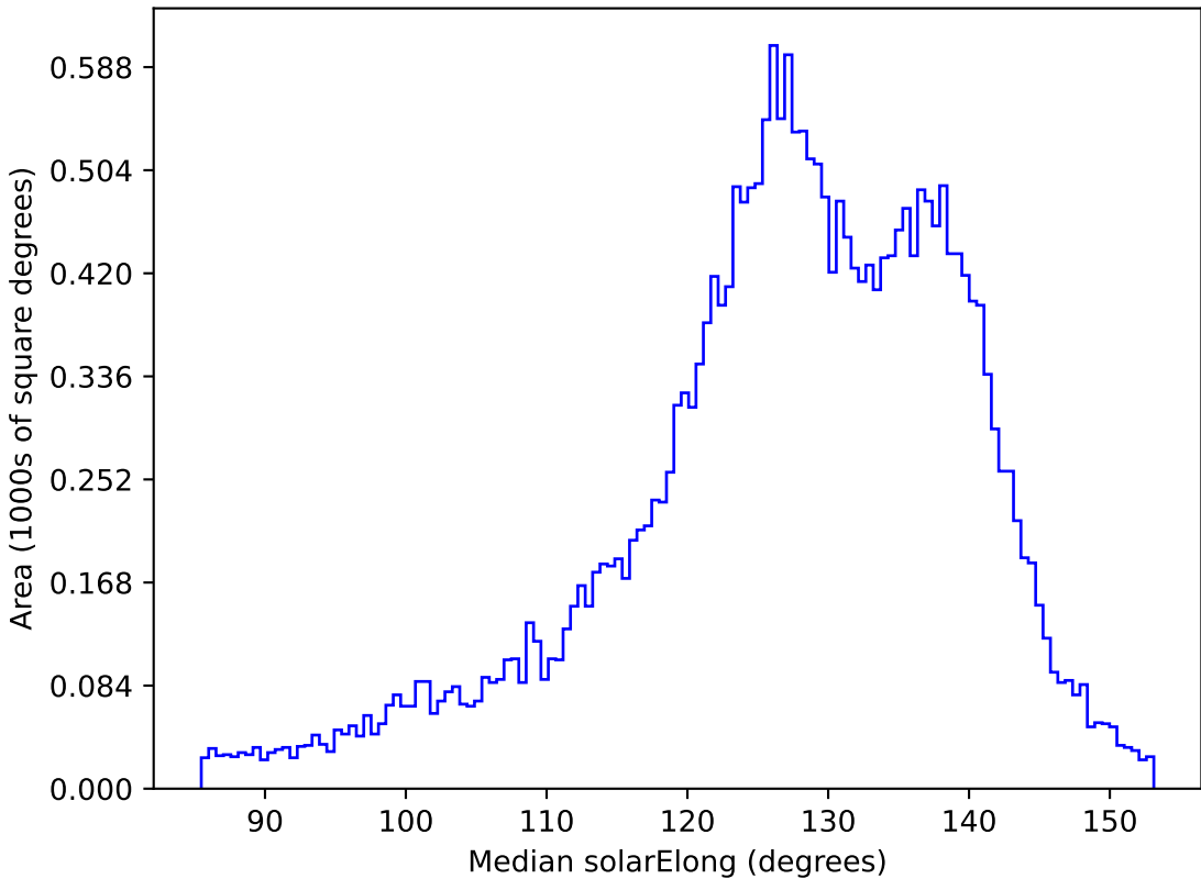
too_elab_r32_d2_gz_v3.4_10yrs All sky z band: Median solarElong
