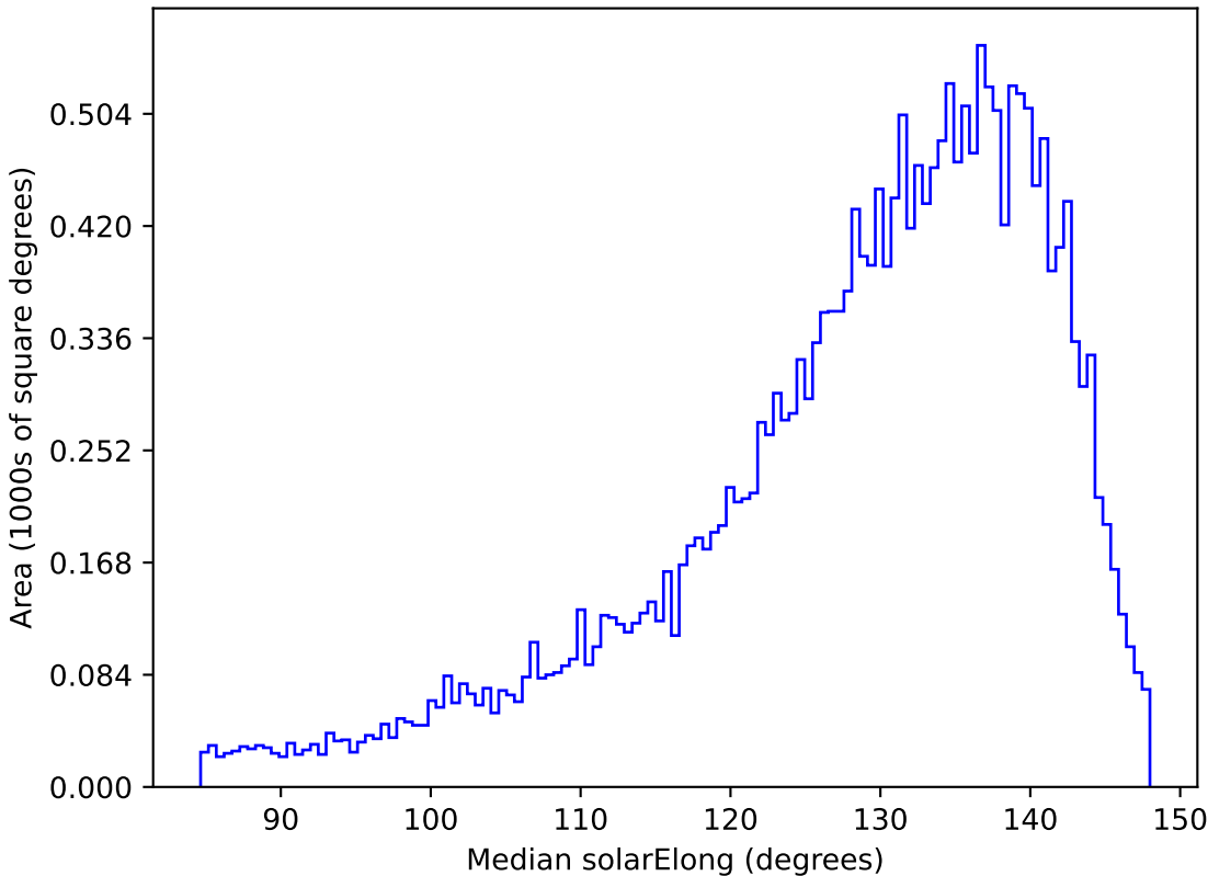
too_elab_r32_d2_gz_v3.4_10yrs All sky y band: Median solarElong
