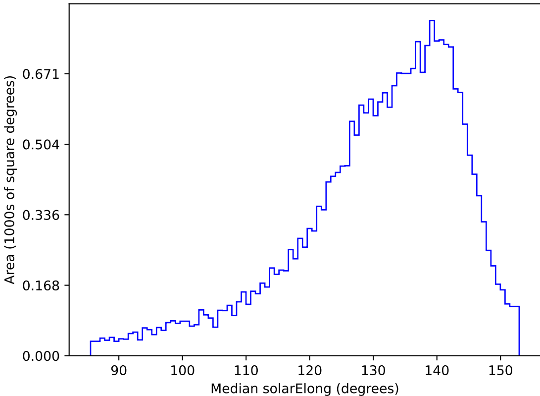
too_elab_r32_d2_gz_v3.4_10yrs All sky r band: Median solarElong
