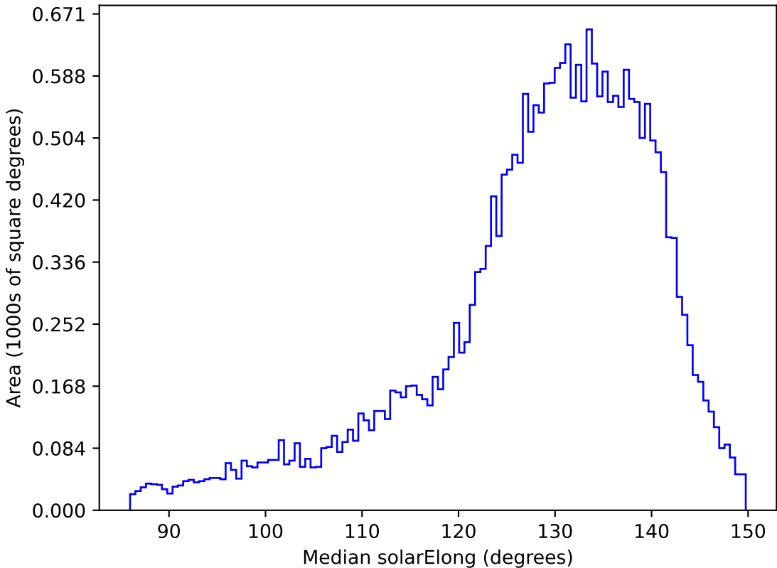
too_elab_r32_d2_gz_v3.4_10yrs All sky i band: Median solarElong
