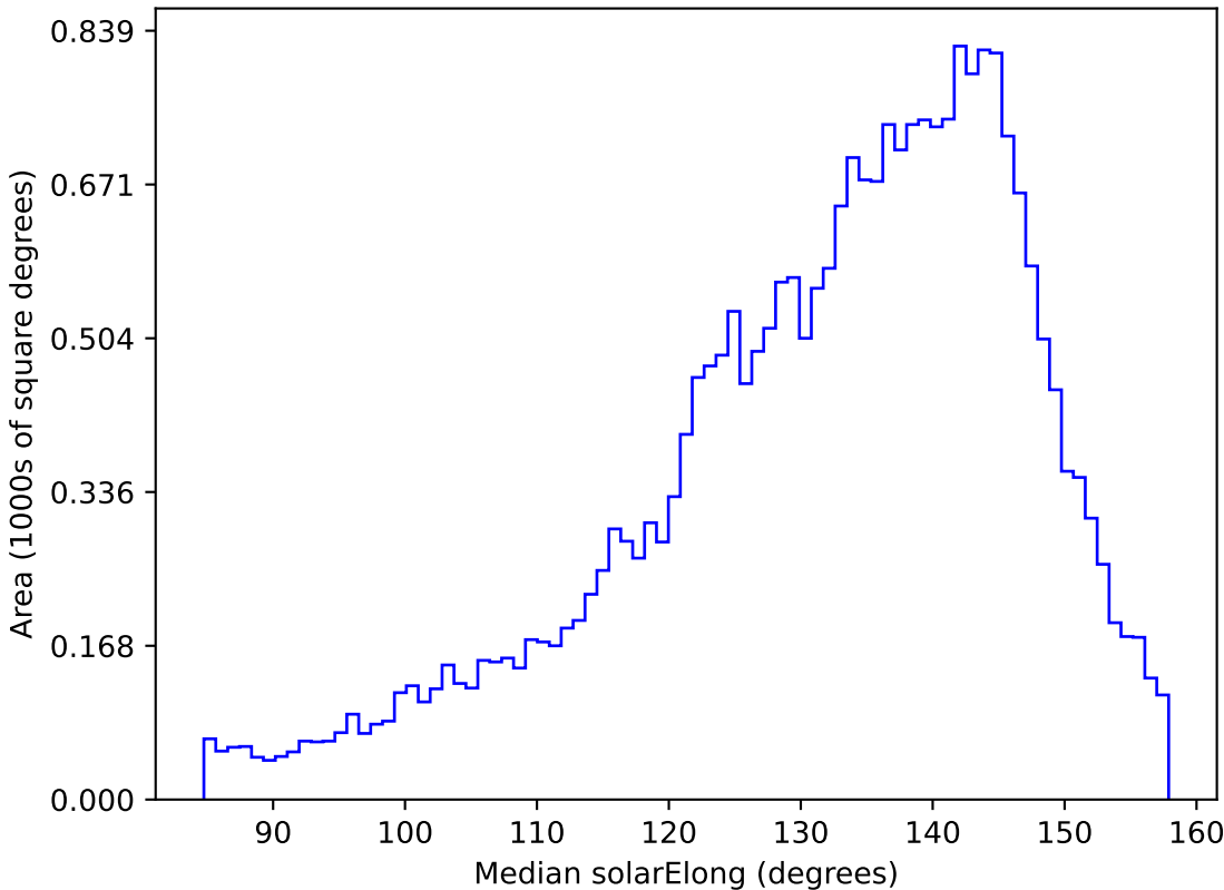
too_elab_r32_d2_gz_v3.4_10yrs All sky g band: Median solarElong
