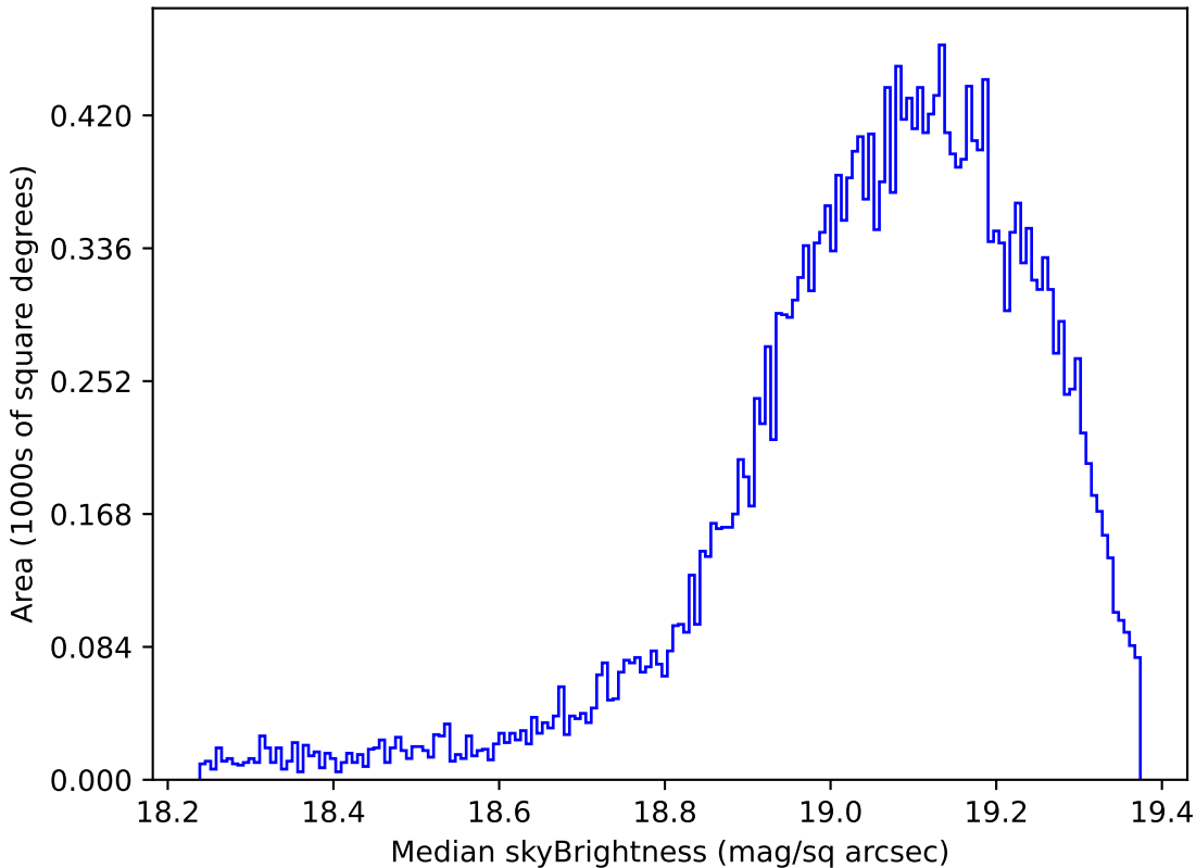
too_elab_r32_d2_gz_v3.4_10yrs Yr 1 z band: Median skyBrightness
