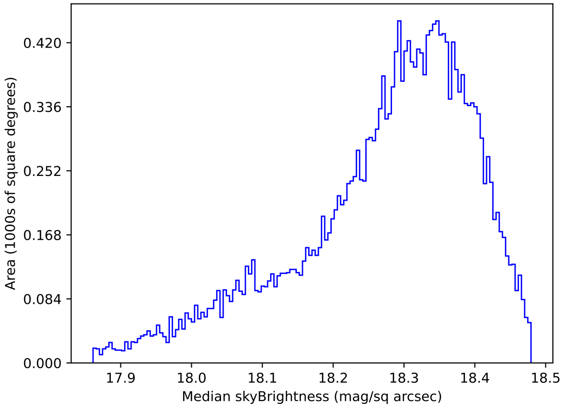
too_elab_r32_d2_gz_v3.4_10yrs Yr 1 y band: Median skyBrightness
