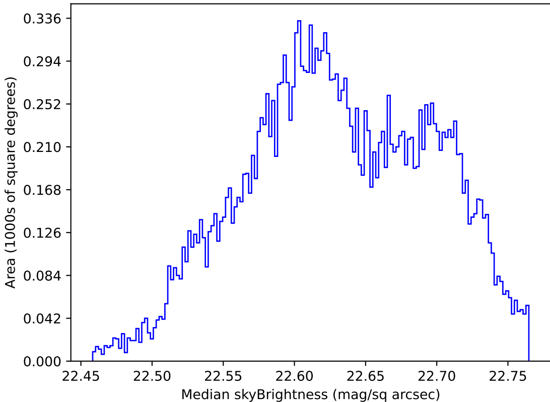
too_elab_r32_d2_gz_v3.4_10yrs Yr 1 u band: Median skyBrightness
