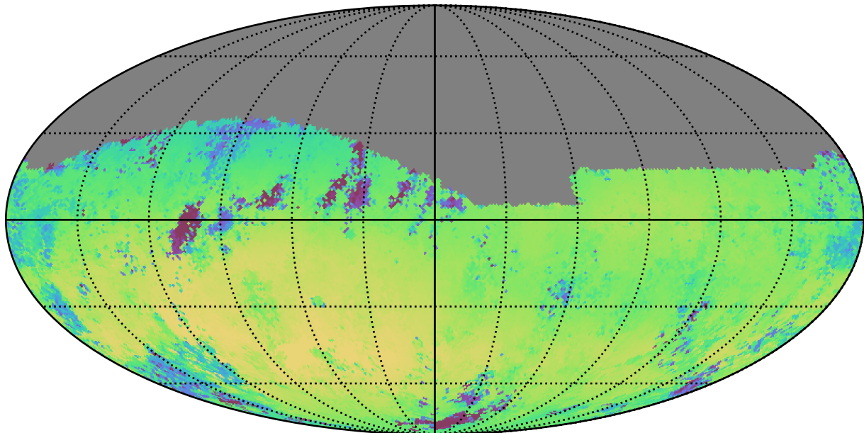
too_elab_r32_d2_gz_v3.4_10yrs Yr 1 r band: Median skyBrightness
