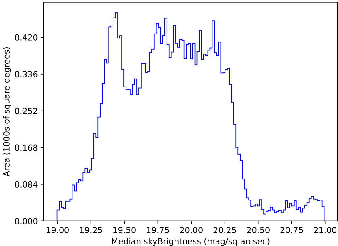
too_elab_r32_d2_gz_v3.4_10yrs Yr 1 all bands: Median skyBrightness
