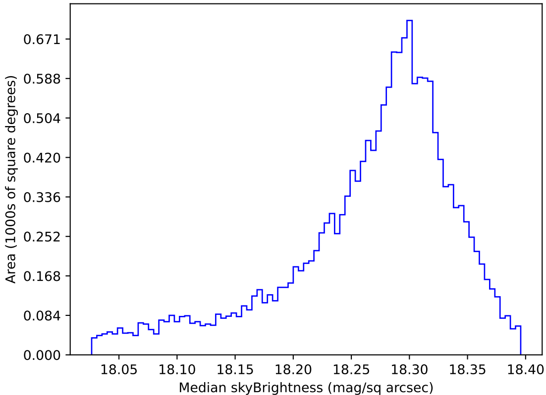
too_elab_r32_d2_gz_v3.4_10yrs WFD y band: Median skyBrightness
