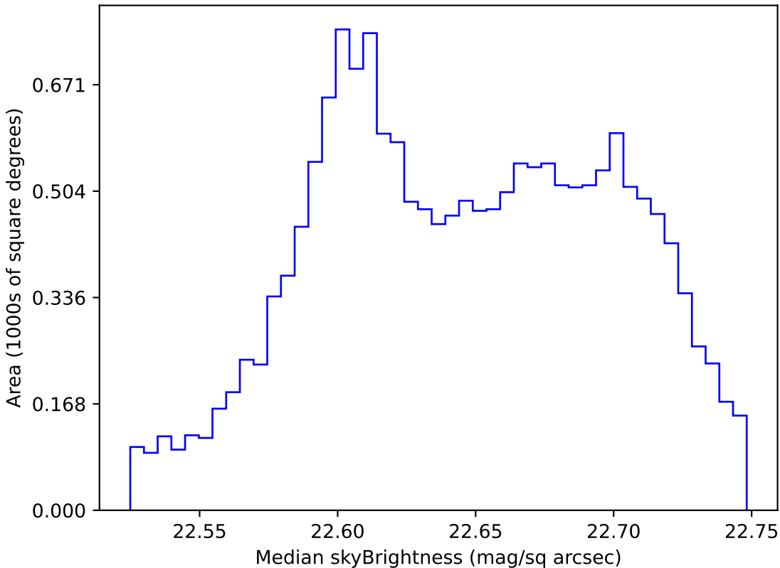
too_elab_r32_d2_gz_v3.4_10yrs WFD u band: Median skyBrightness
