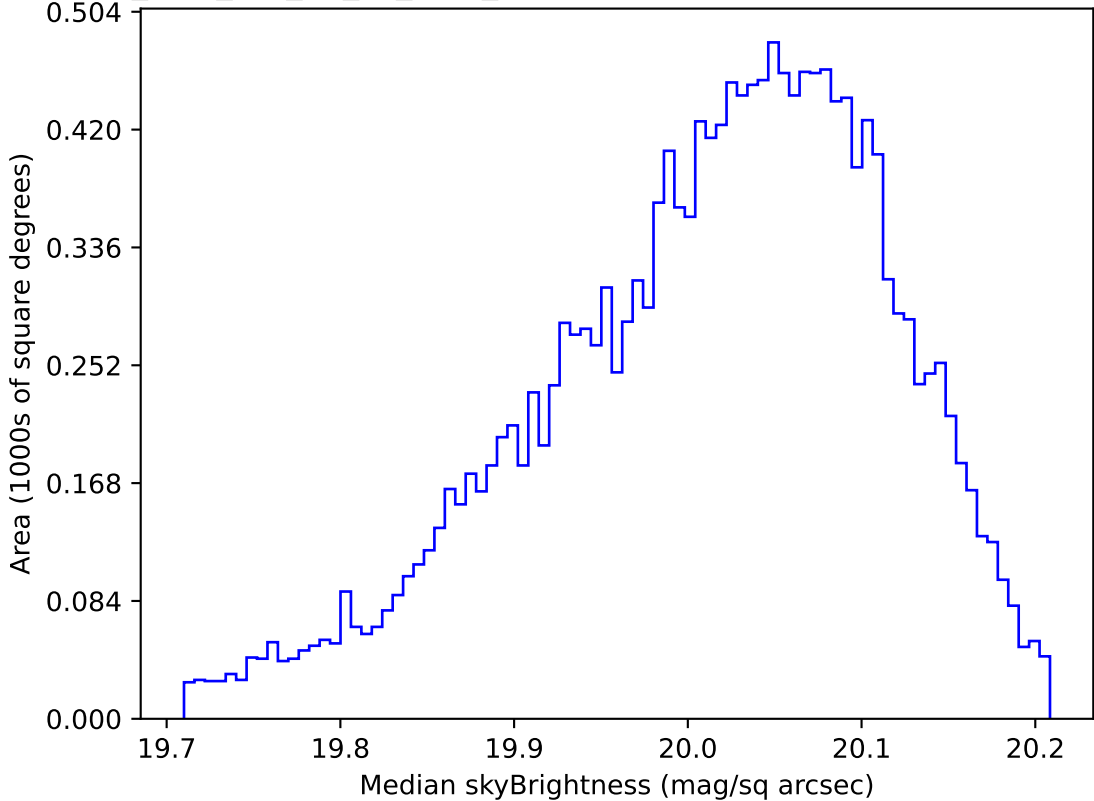
too_elab_r32_d2_gz_v3.4_10yrs WFD i band: Median skyBrightness
