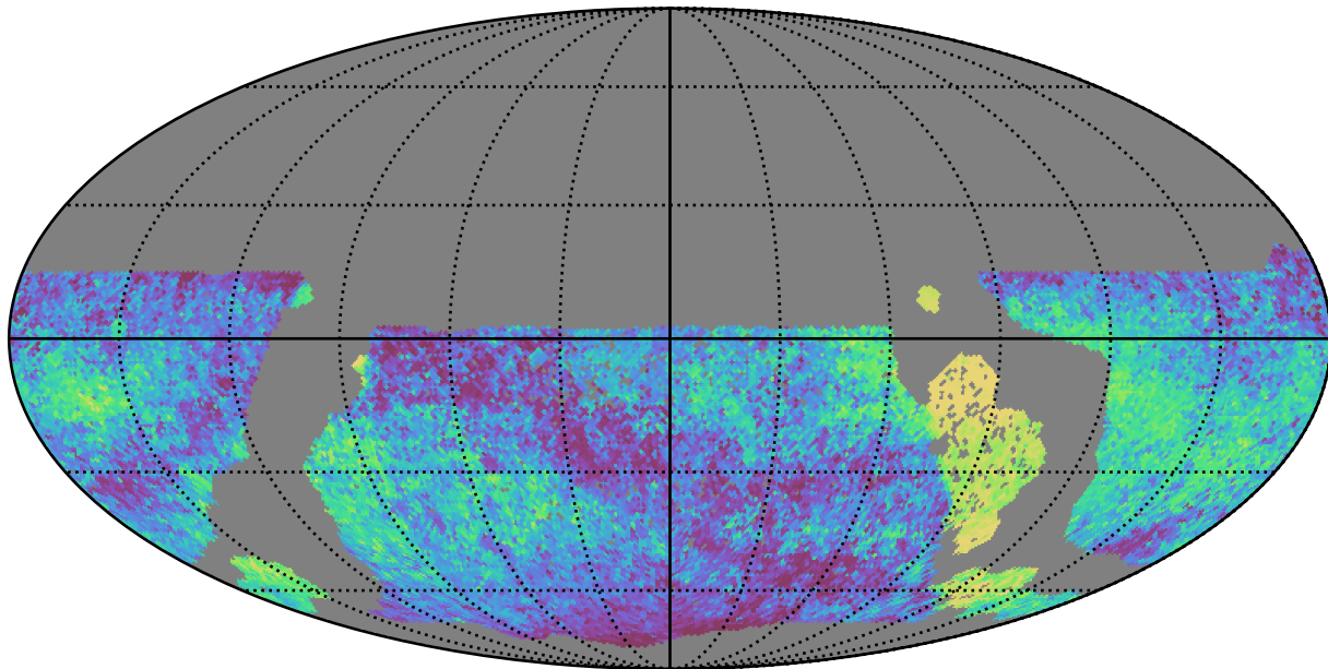
too_elab_r32_d2_gz_v3.4_10yrs WFD all bands: Median skyBrightness
