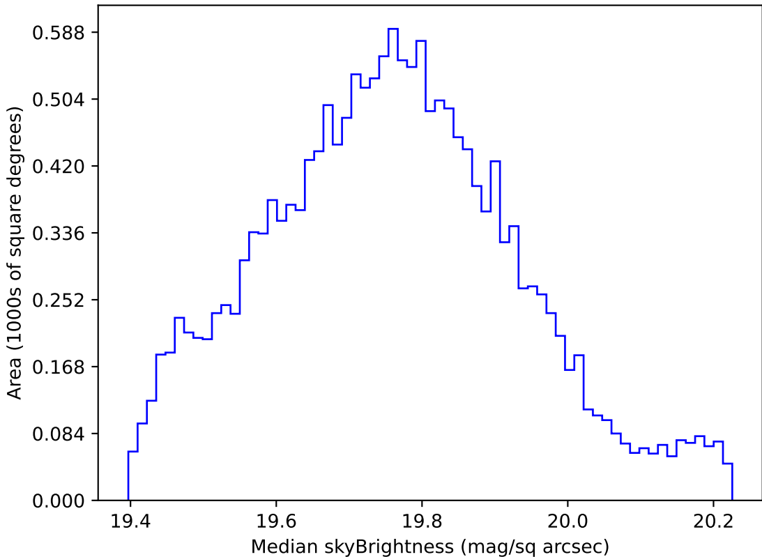
too_elab_r32_d2_gz_v3.4_10yrs WFD all bands: Median skyBrightness
