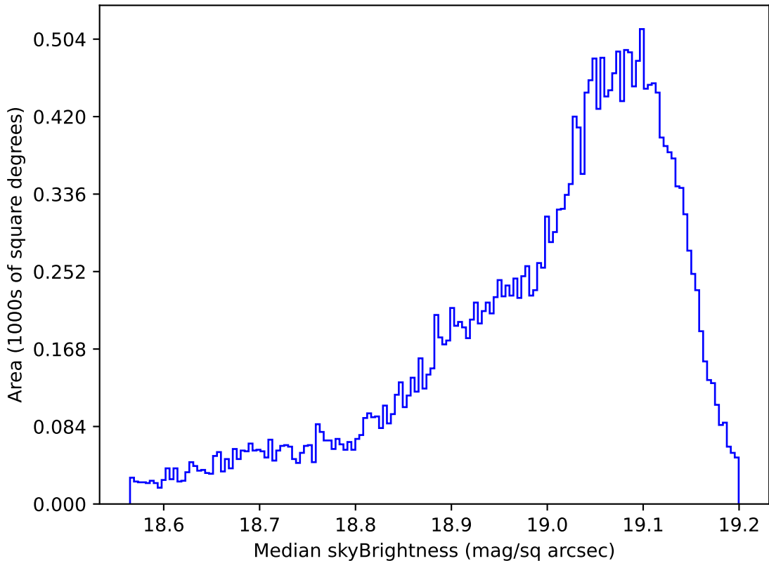
too_elab_r32_d2_gz_v3.4_10yrs All sky z band: Median skyBrightness
