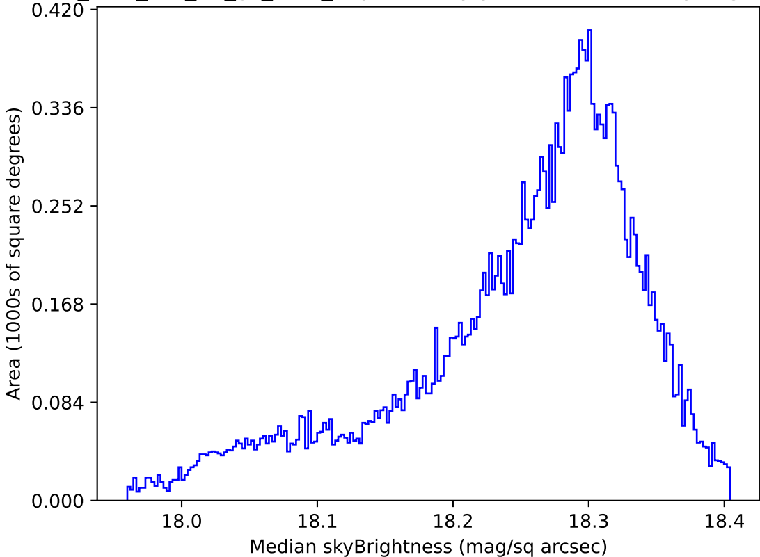
too_elab_r32_d2_gz_v3.4_10yrs All sky y band: Median skyBrightness
