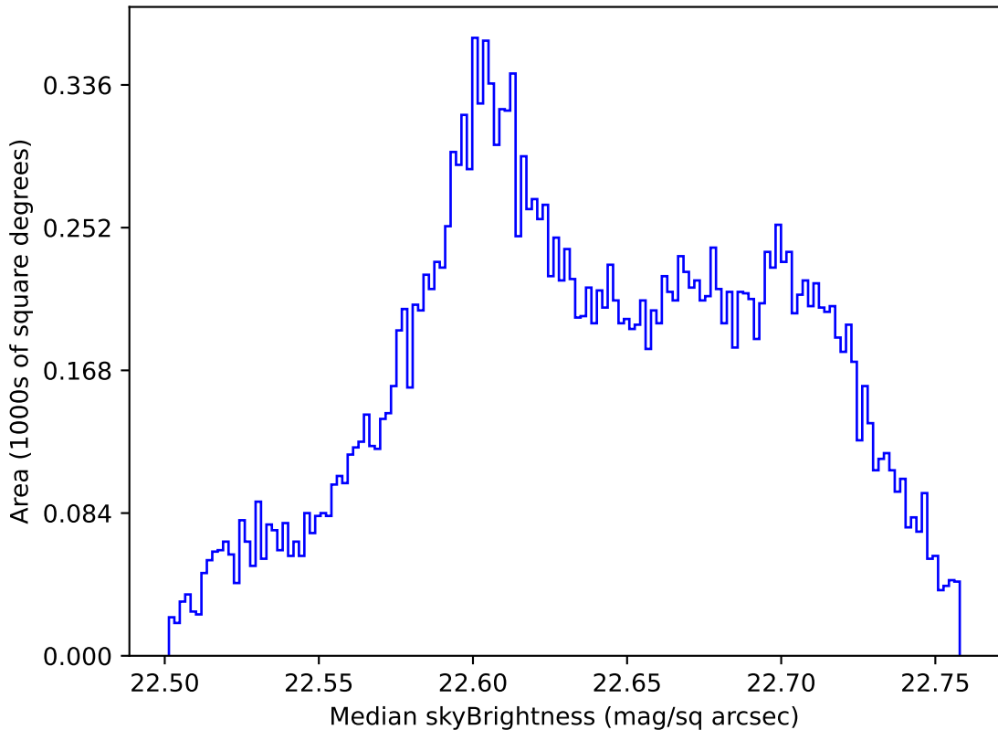
too_elab_r32_d2_gz_v3.4_10yrs All sky u band: Median skyBrightness
