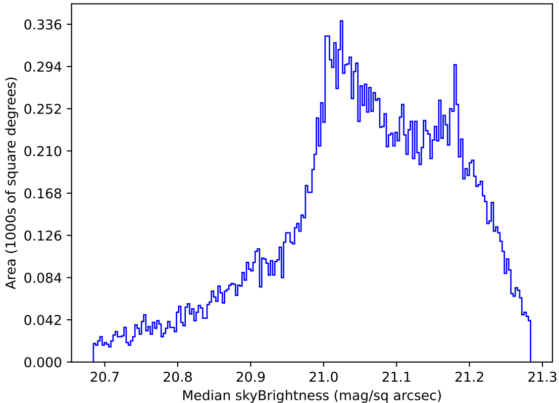
too_elab_r32_d2_gz_v3.4_10yrs All sky r band: Median skyBrightness
