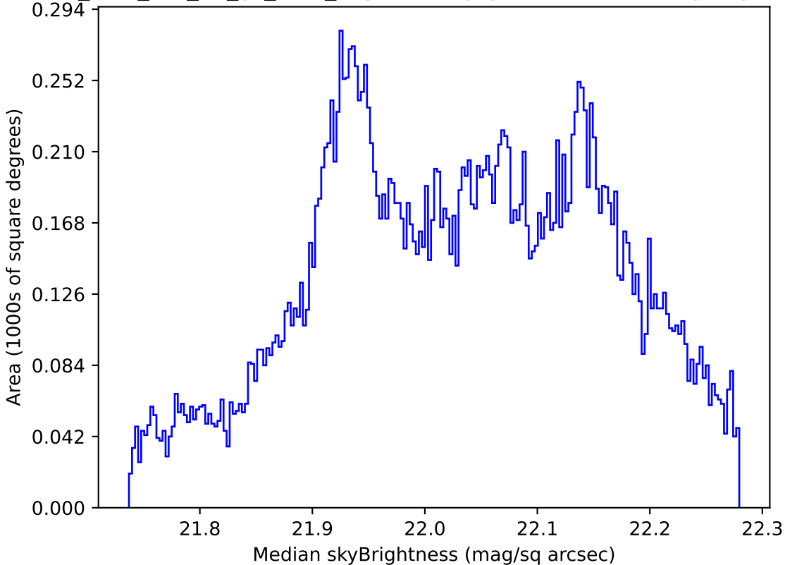
too_elab_r32_d2_gz_v3.4_10yrs All sky g band: Median skyBrightness
