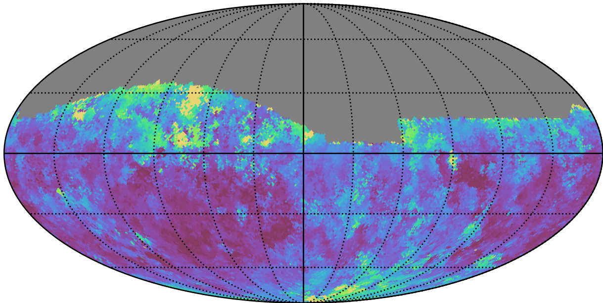
too_elab_r32_d2_gz_v3.4_10yrs Yr 1 z band: Median seeingGeom
