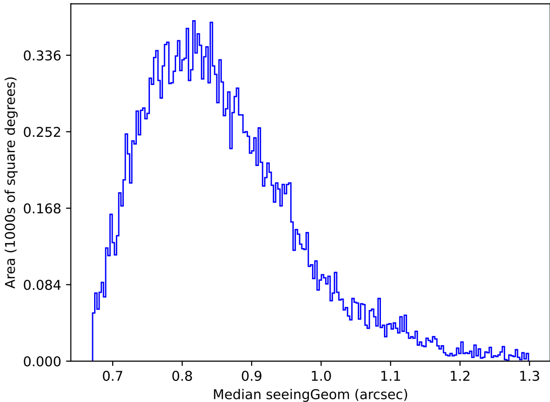
too_elab_r32_d2_gz_v3.4_10yrs Yr 1 z band: Median seeingGeom
