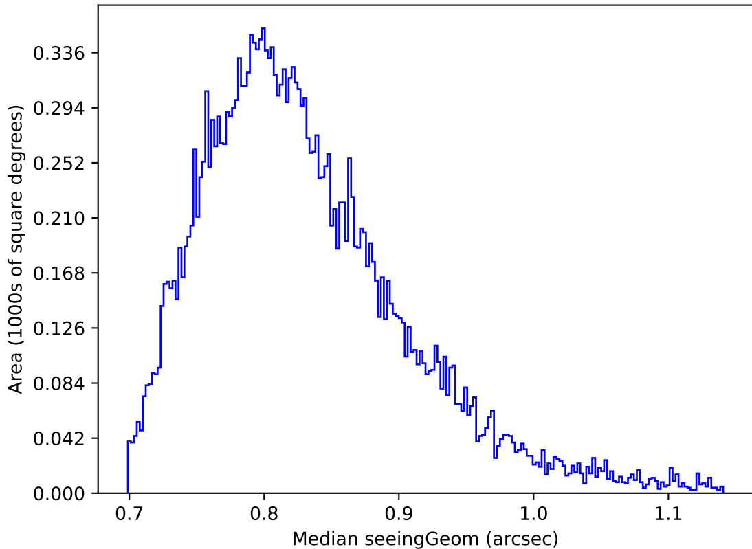
too_elab_r32_d2_gz_v3.4_10yrs Yr 1 y band: Median seeingGeom
