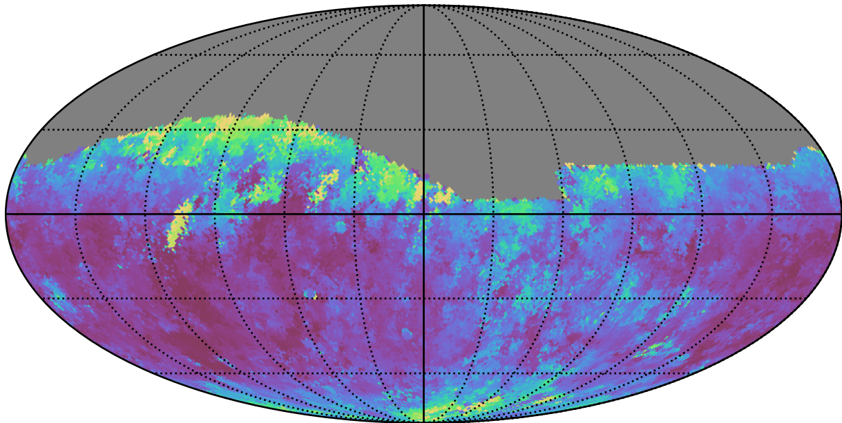
too_elab_r32_d2_gz_v3.4_10yrs Yr 1 r band: Median seeingGeom
