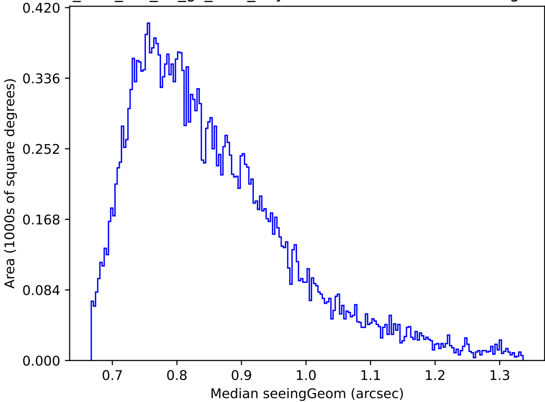
too_elab_r32_d2_gz_v3.4_10yrs Yr 1 r band: Median seeingGeom
