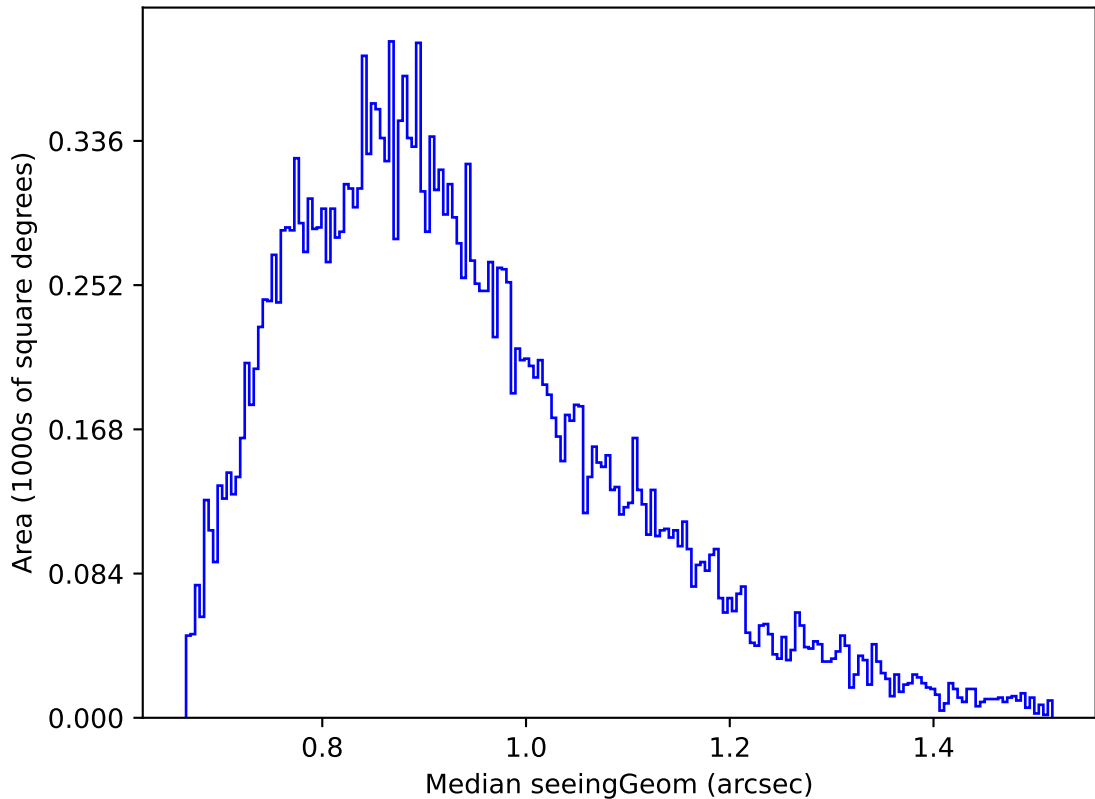
too_elab_r32_d2_gz_v3.4_10yrs Yr 1 g band: Median seeingGeom
